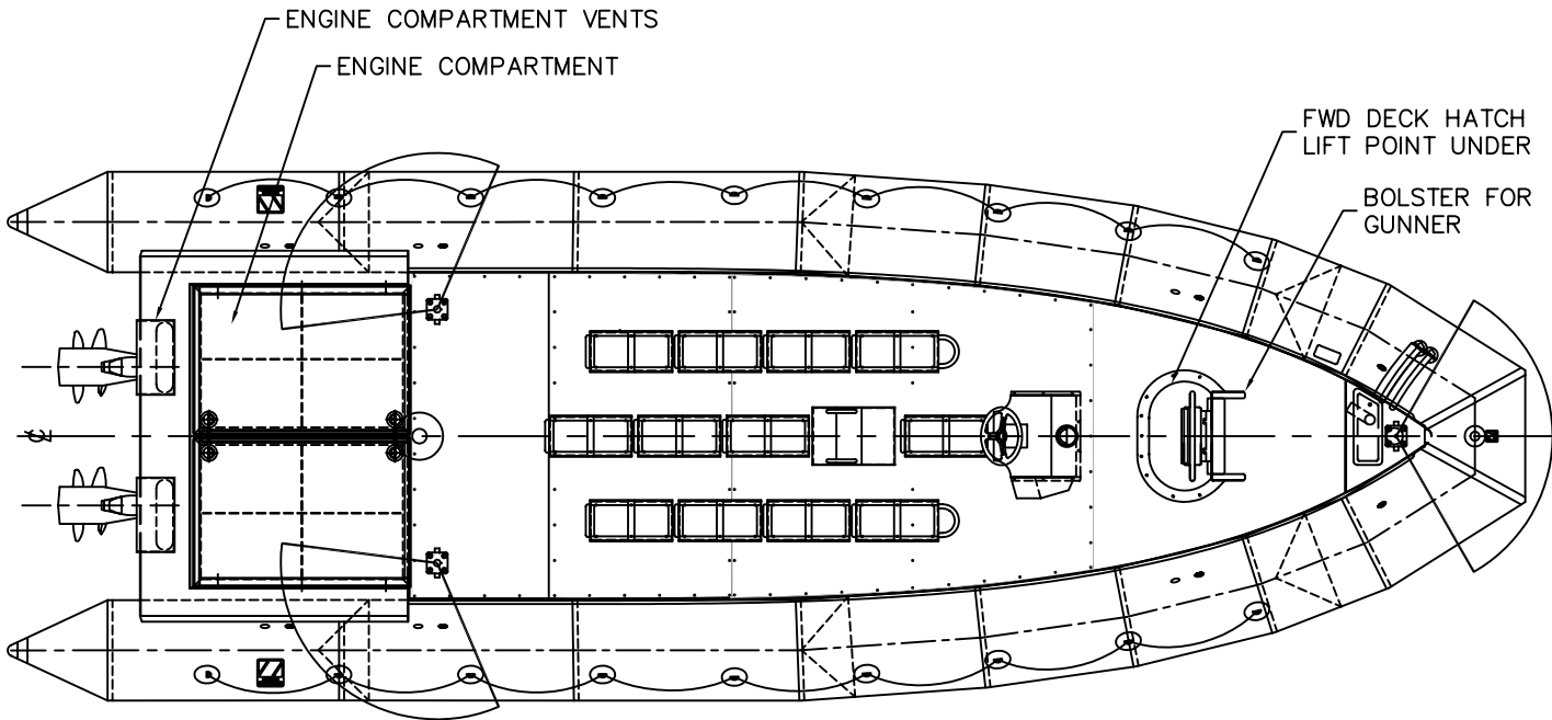
H923 AFT IO - PLAN DETAIL "6-D"
