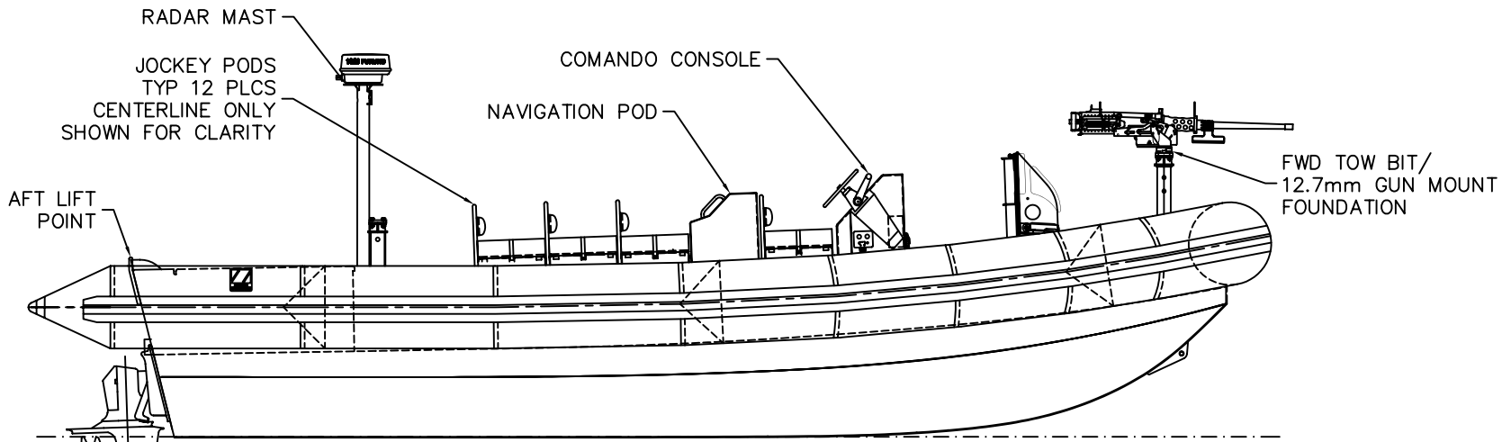
H923 AFT IO - PROFILE DETAIL "6-B"
